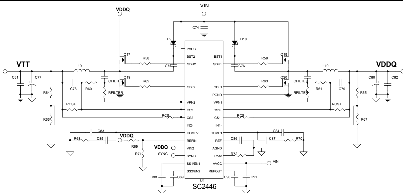
DDR Memory Applications (Separate Input Voltage)
