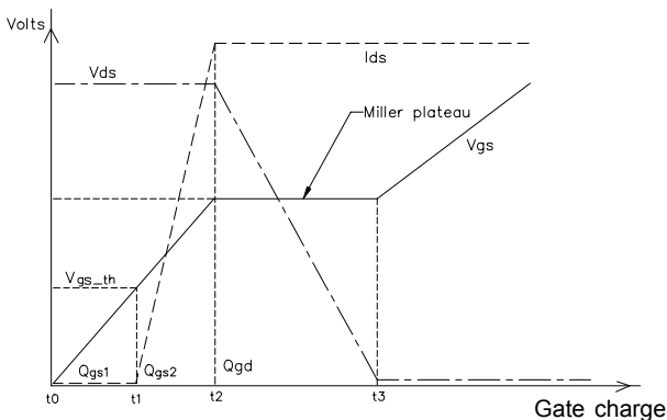
Figure 11. MOSFET switching characteristics
