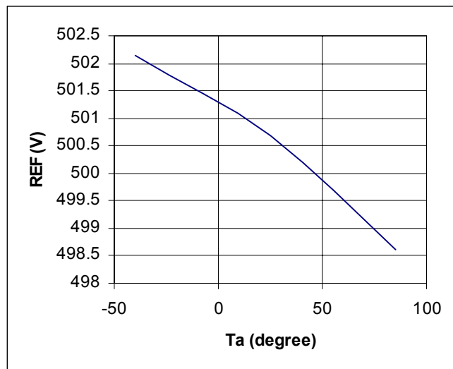
REF Voltage vs. Temperature
