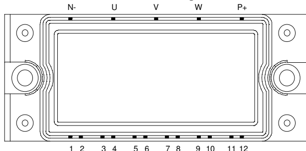
Pin out: APTGF50X120P2 (Short pins)
