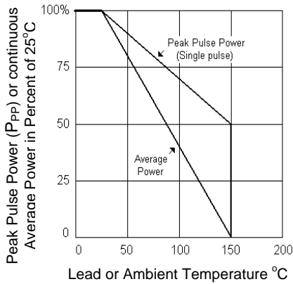
FIGURE 3 Derating Curve
