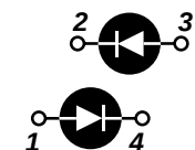
Anti-Parallel APT2X100D120J
