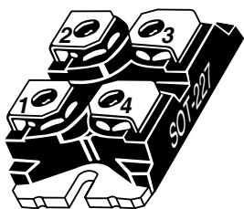
Parallel APT2X101D40J
