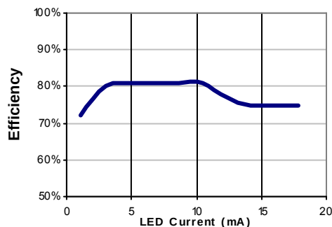
Figure 10: Efficiency vs. LED Output Current.
