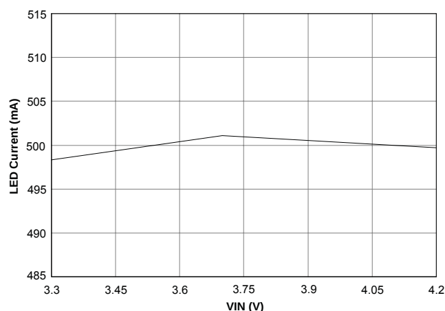
Spotlight Current, R_{ISET} = 750m\Omega , V_{OUT} = 2.93V
