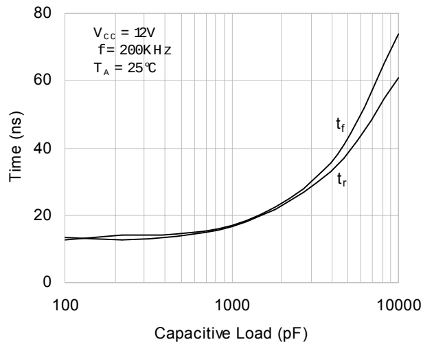
Rise and Fall Time vs. Capacitive Load
