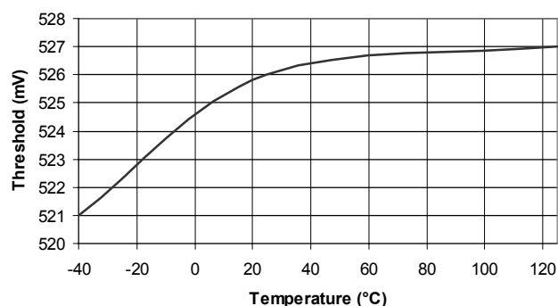
Current Limit Threshold vs Temperature
