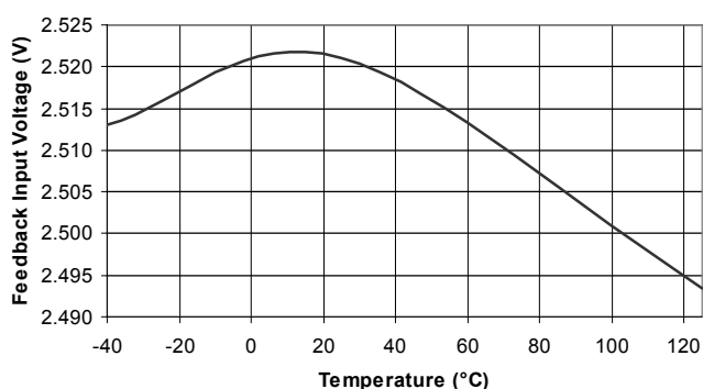
Error Amplifier Feedback Voltage vs Temperature
