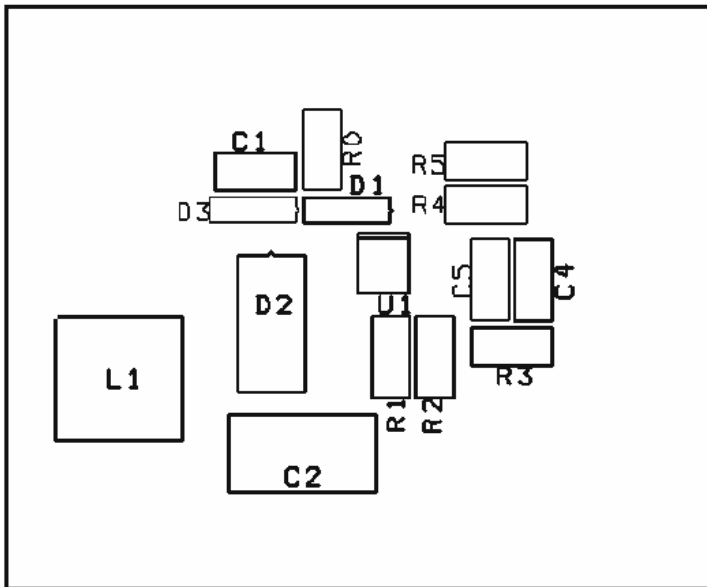
(COMPONENT - TOP)
