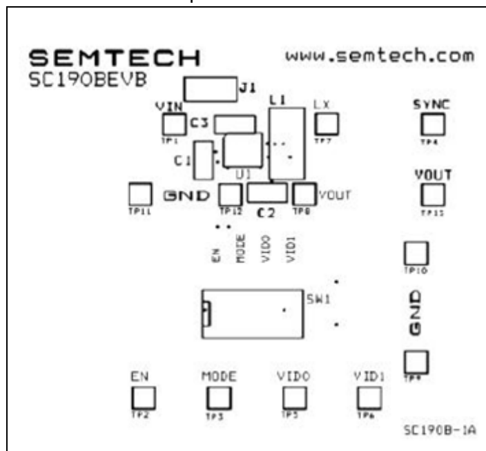
Top Silkscreen
