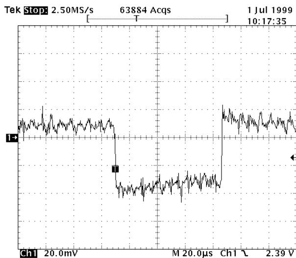
Transient Response V_o = 2.4V , I_o = 300mA to 15A
