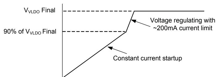
Figure 10 — LDO Start-Up
