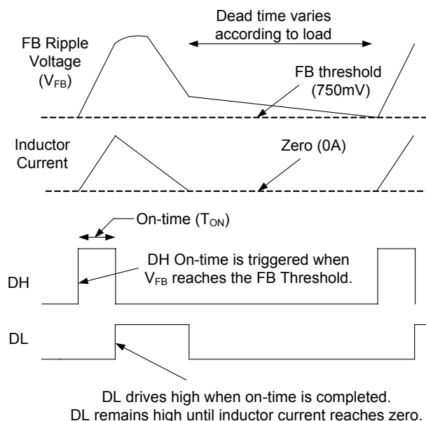
Figure 6 — Power-save Operation
