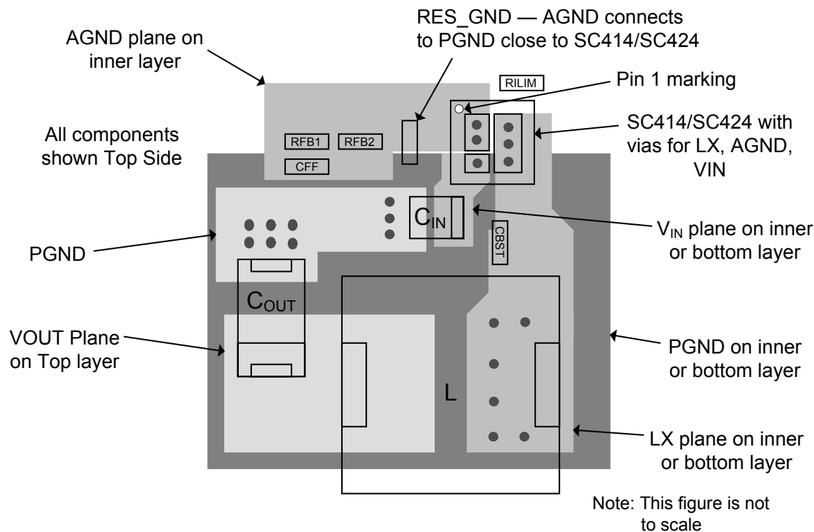
Figure 15 — PCB Layout
