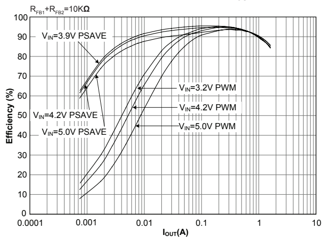
Efficiency vs. Load Current V_{OUT} = 3.3V
