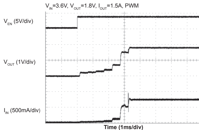
PWM Start-up
