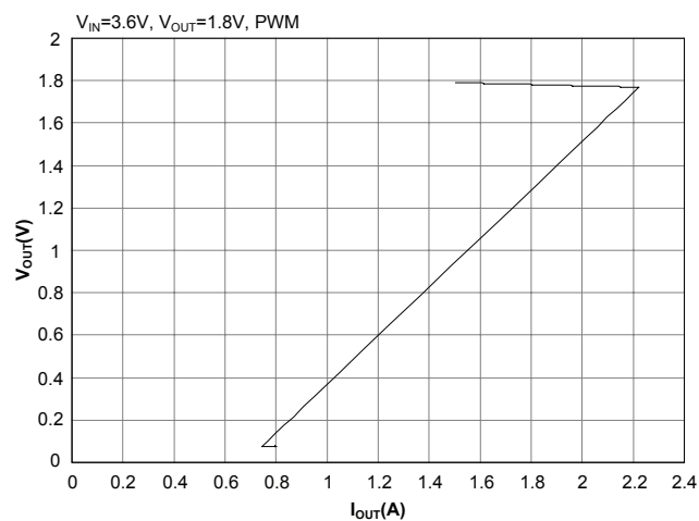
Current Limit
