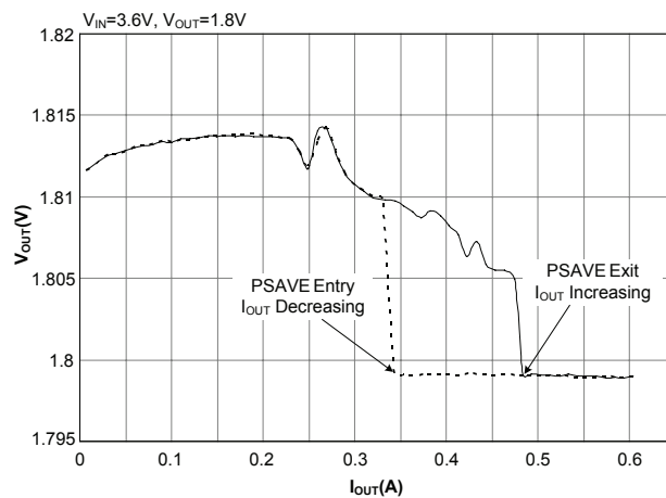
PWM to PSAVE Hysteresis
