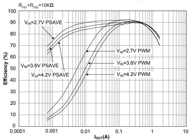
Efficiency vs. Load Current V_{OUT} = 1.8V
