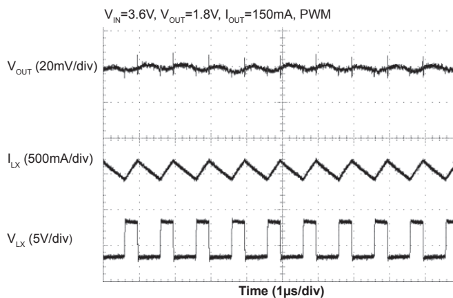
PWM Operation
