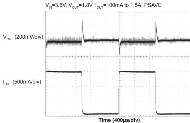
Load Transient Response-4
