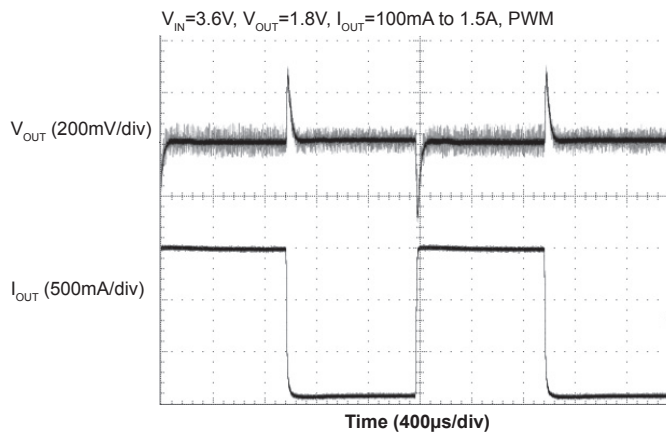
Load Transient Response-2
