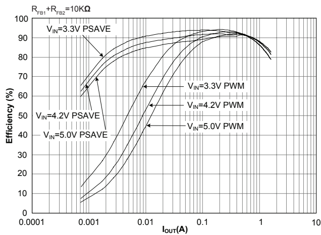
Efficiency vs. Load Current V_{OUT} = 2.5V
