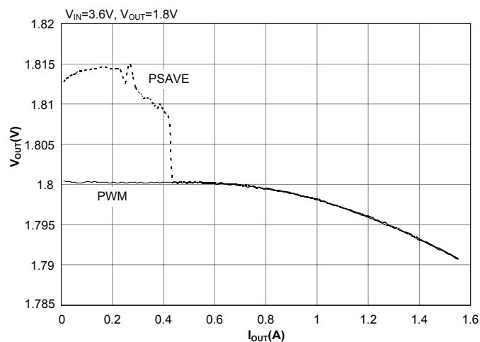
Load Regulation
