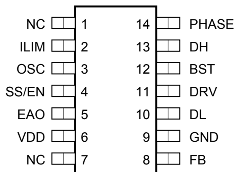
(14 Pin SOIC)
