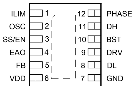
(12 Pin MLPD)
