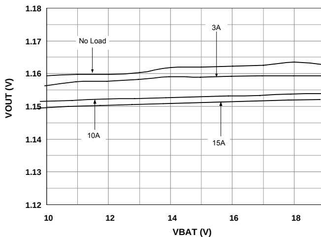
Line Regulation
