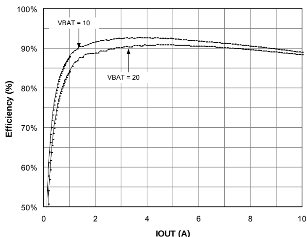
2.5V Efficiency vs. Output Current Continuous Conduction Mode
