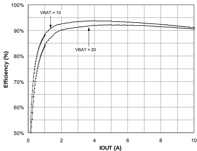
1.5V Efficiency vs. Output Current Continuous Conduction Mode
