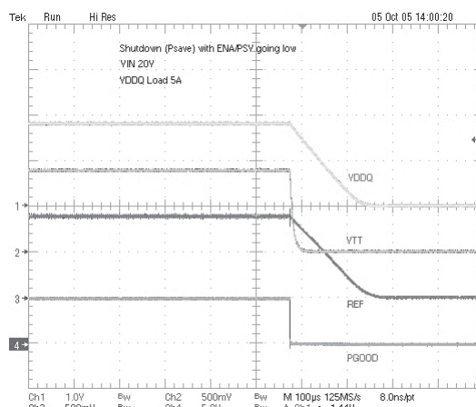
Startup (PSV), EN/PSV Going Low, VDDQ = 5A
