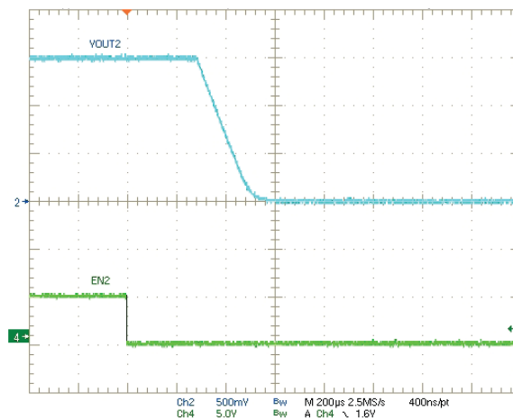
Shutdown VOUT2, 1.5V 2A Load
