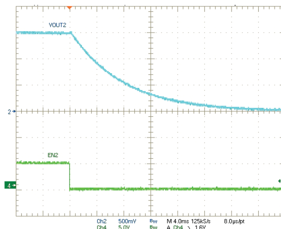
Shutdown VOUT2, 1.5V No Load
