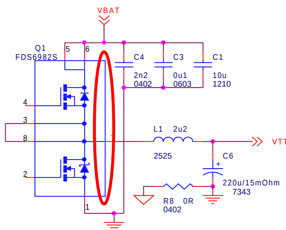
Figure 7: Power Section and Input Loop
