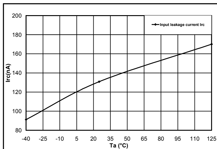
RC pin leakage current vs. Temperature
