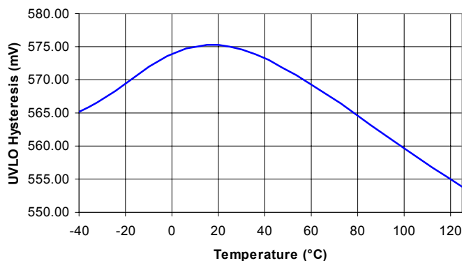
(Sc4910A) UVLO Hysteresis vs Temperature
