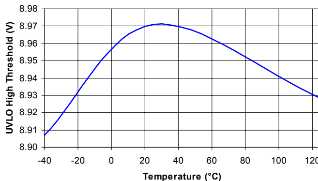
(Sc4910A) UVLO High Threshold vs Temperature
