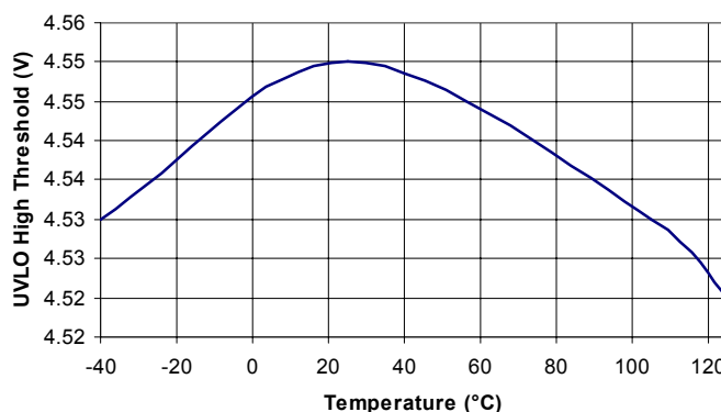
(Sc4910B) UVLO High Threshold vs Temperature
