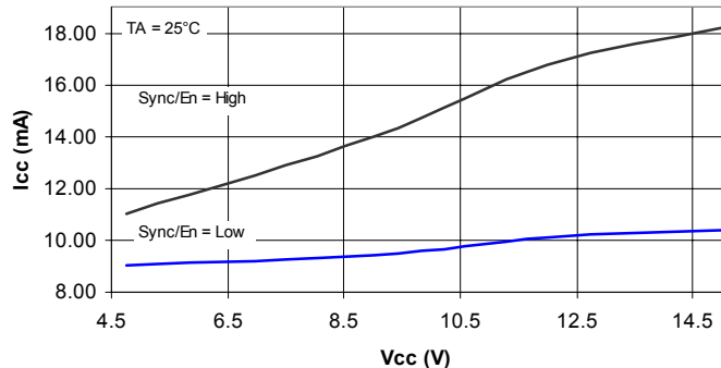
I CC vs V CC
