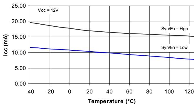
I CC vs Temperature
