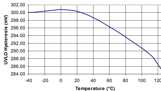
(Sc4910B) UVLO Hysteresis vs Temperature
