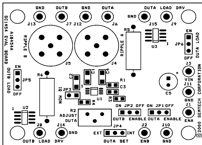
Top Assembly
