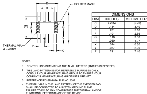
Figure 8. Land Pattern
