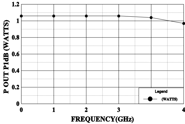
POWER OUTPUT vs FREQUENCY
