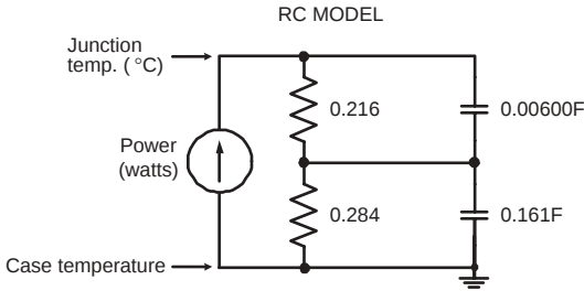
FIGURE 19B, TRANSIENT THERMAL IMPEDANCE MODEL
