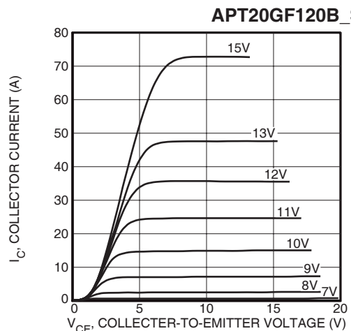
FIGURE 2, Output Characteristics ( T_J = 125^\circ\text{C} )
