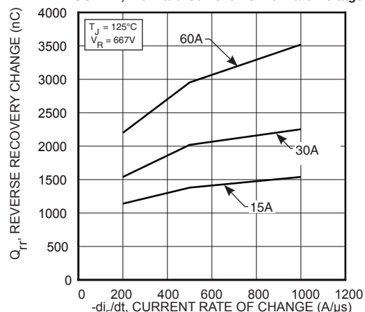
FIGURE 4, Reverse Recovery Change vs. Current Rate of Change
