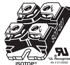
ISOTOP® APT47GA60JD40
