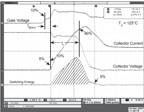
Figure 20, Turn-on Switching Waveforms and Definitions
