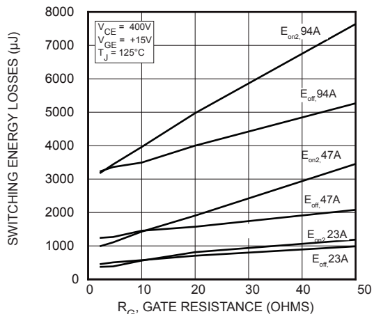
FIGURE 15, Switching Energy Losses vs Gate Resistance
