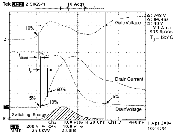
Figure 18, Turn-on Switching Waveforms and Definitions
