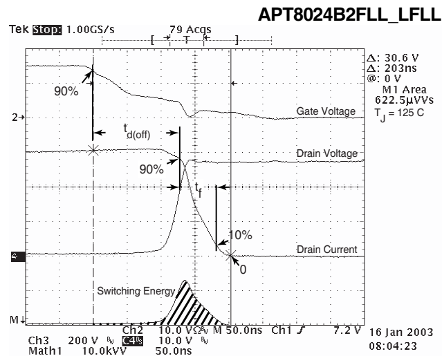
Figure 19, Turn-off Switching Waveforms and Definitions
