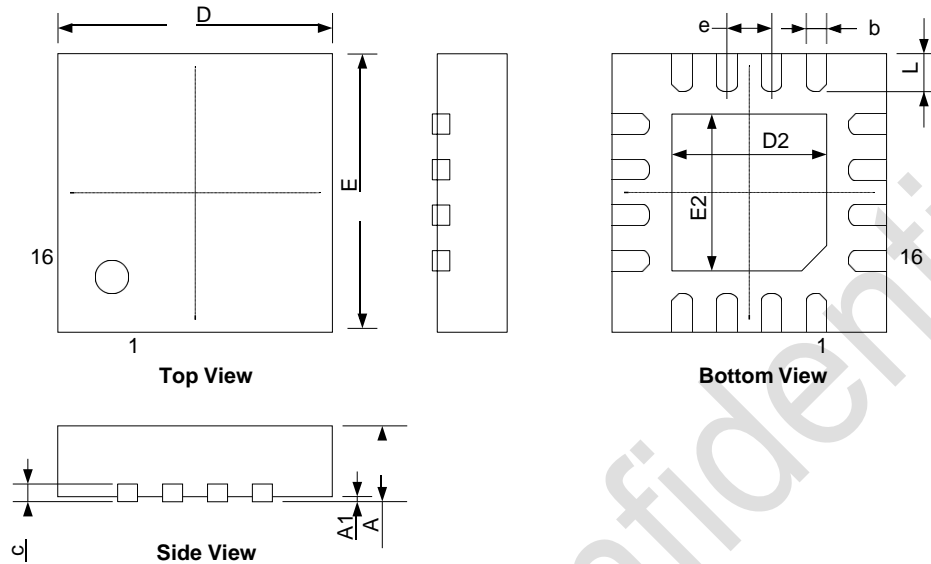
Figure12. 16-Pin QFN 3x3 packaging
