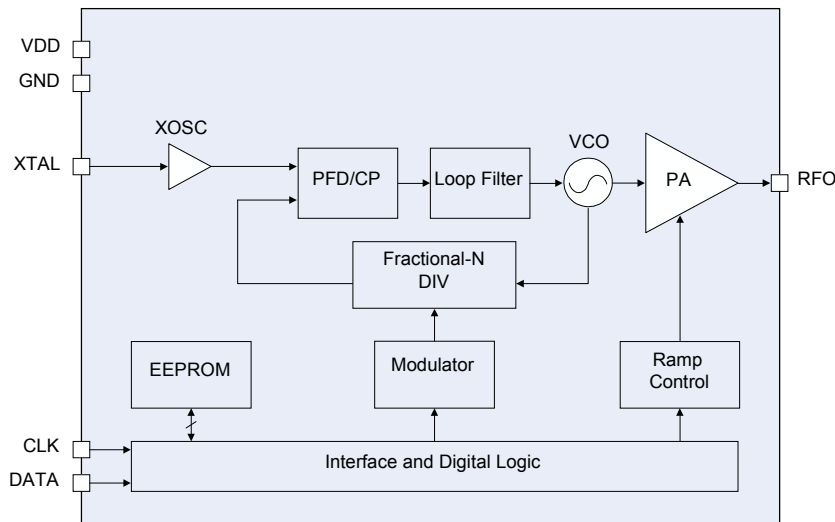
Figure 11. RFM119/RFM119S Functional Block Diagram
