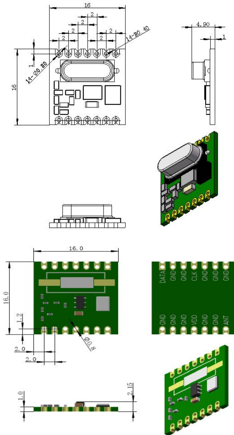
Figure 18 S1/S2 Package Outline Drawing
