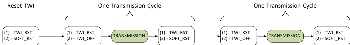
Figure 19. RFM119/S Operation Flow with TWI
